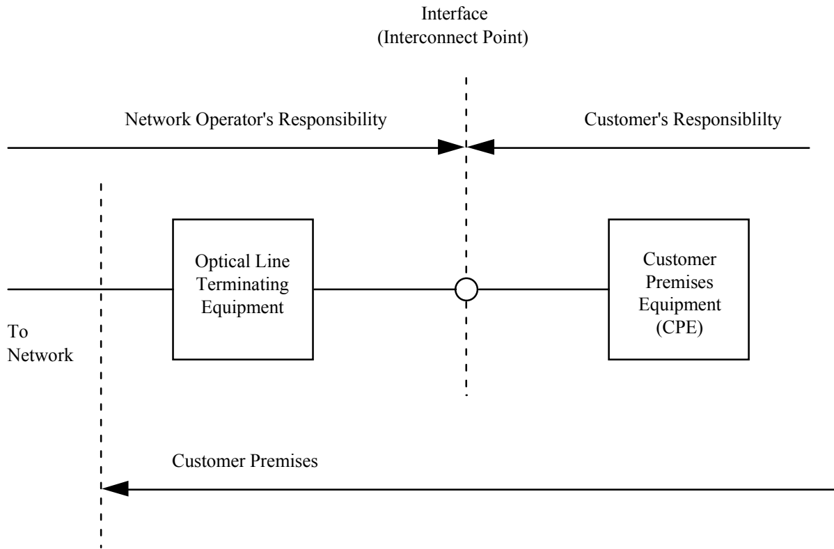
Figure 1 - Interconnection of CPE to the optical leased circuit with SONET interface
